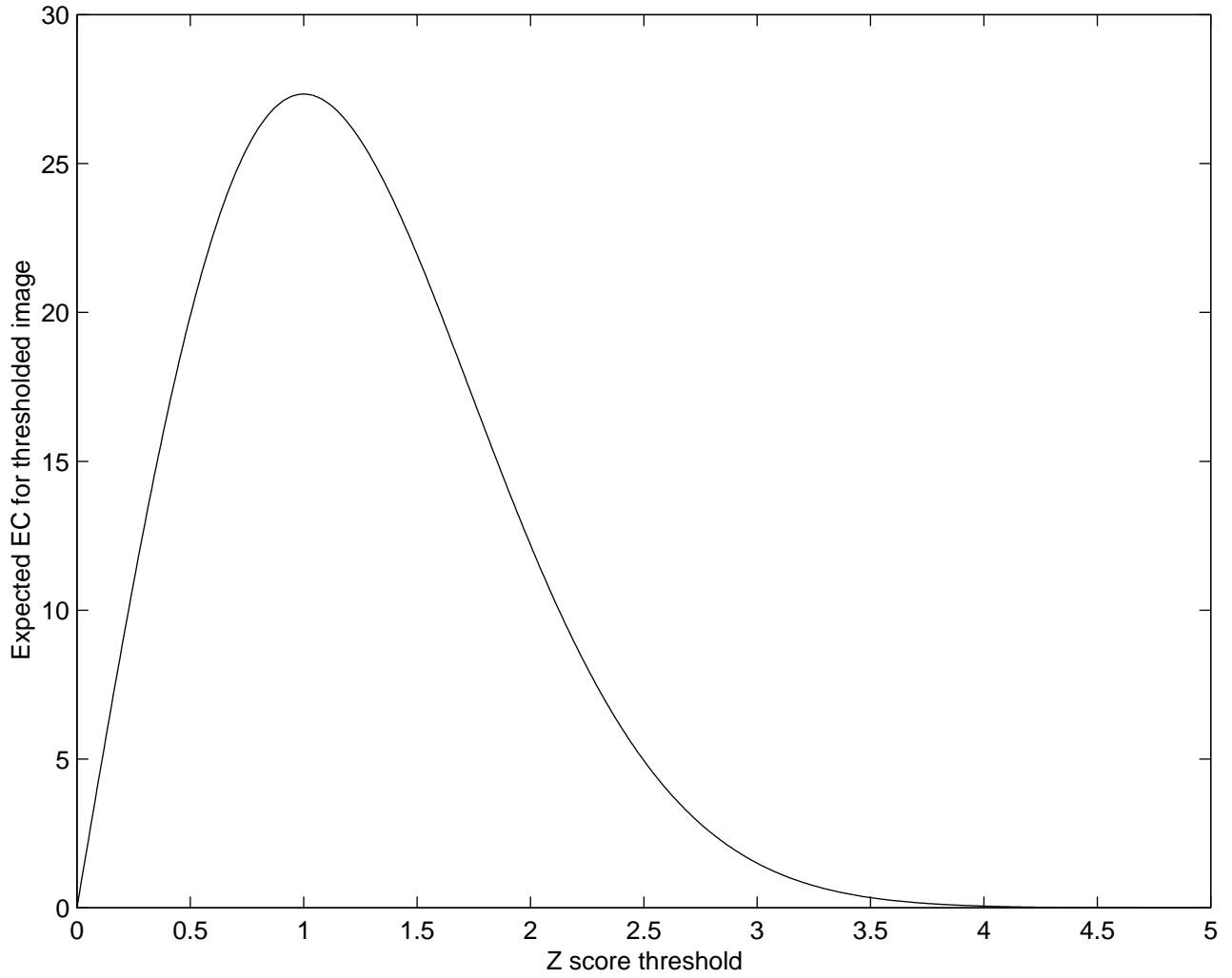
Expected EC for smoothed image with 256 resels
