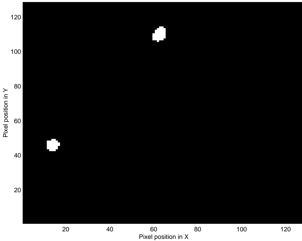
Smoothed image thresholded at Z > 2.75
