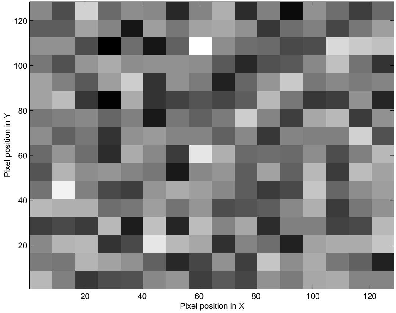
Taking means over 8 by 8 elements from image 1
