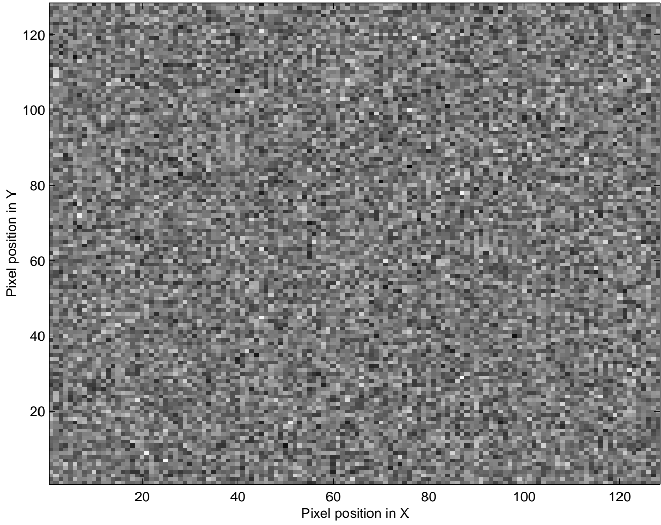
Image 1 – array of independent random numbers
