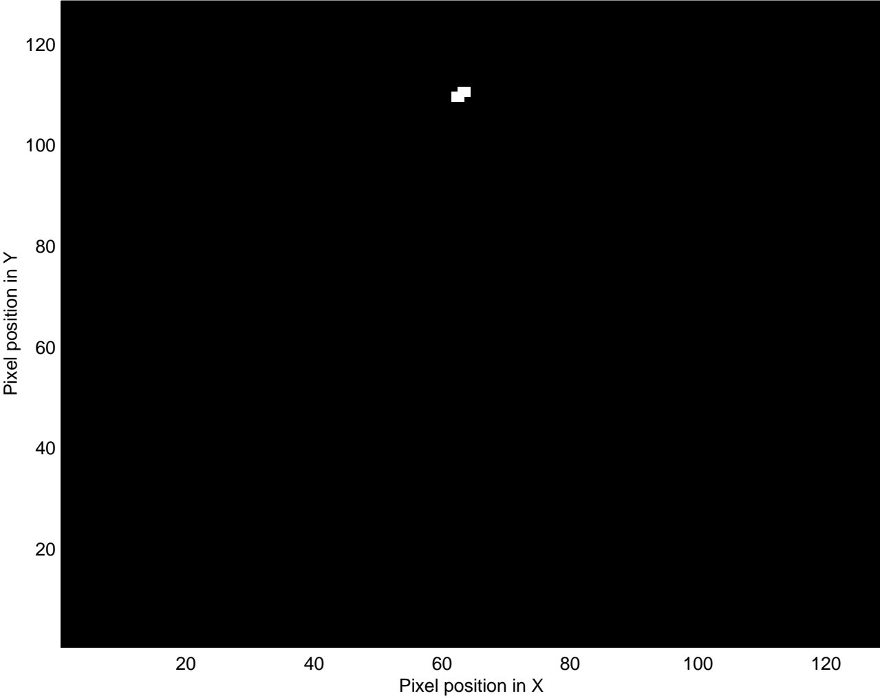
Smoothed image thresholded at Z > 3.5
